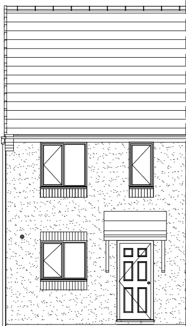
FRONT ELEVATION
