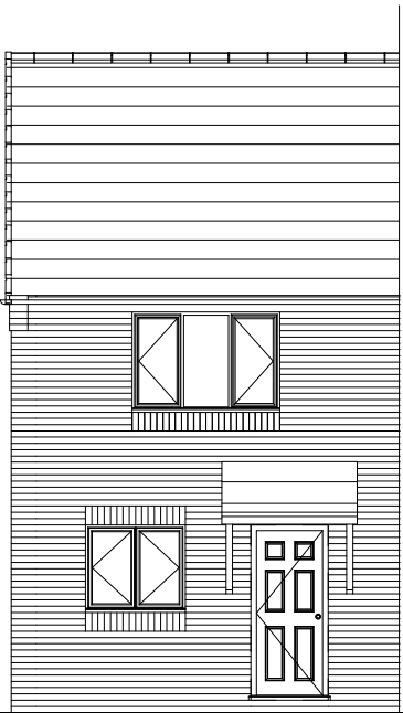
FRONT ELEVATION
