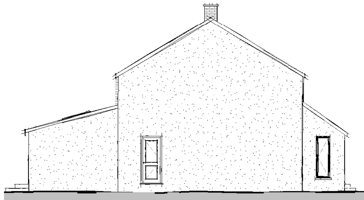
Side Elevation 02
