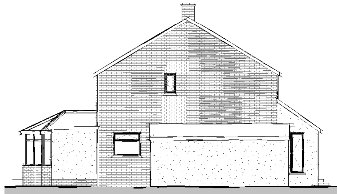
Side Elevation 02
