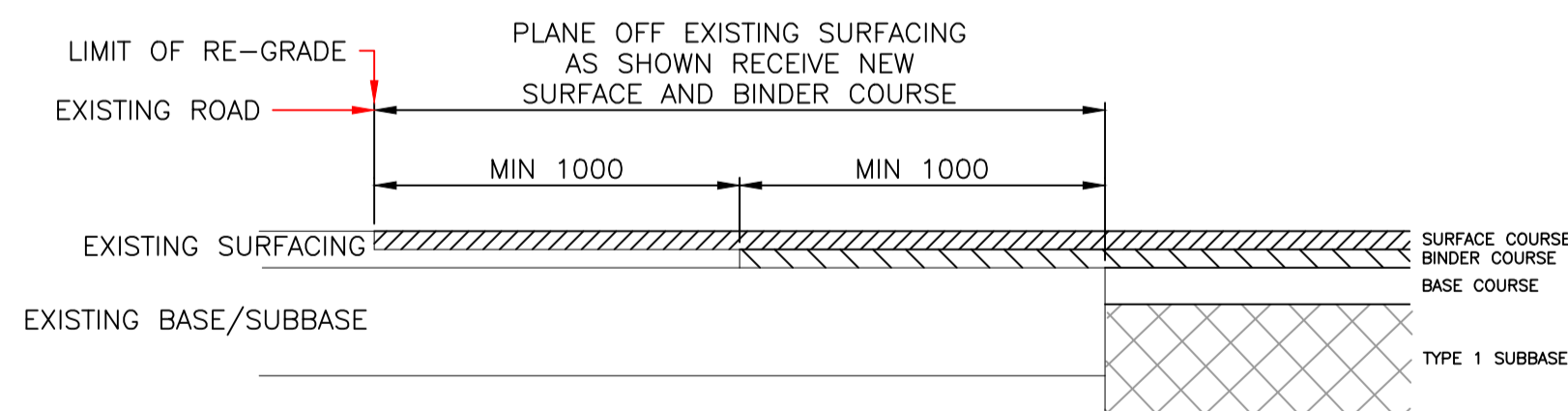
SECTION THROUGH EX. ROAD AT NEW JUNCTION
