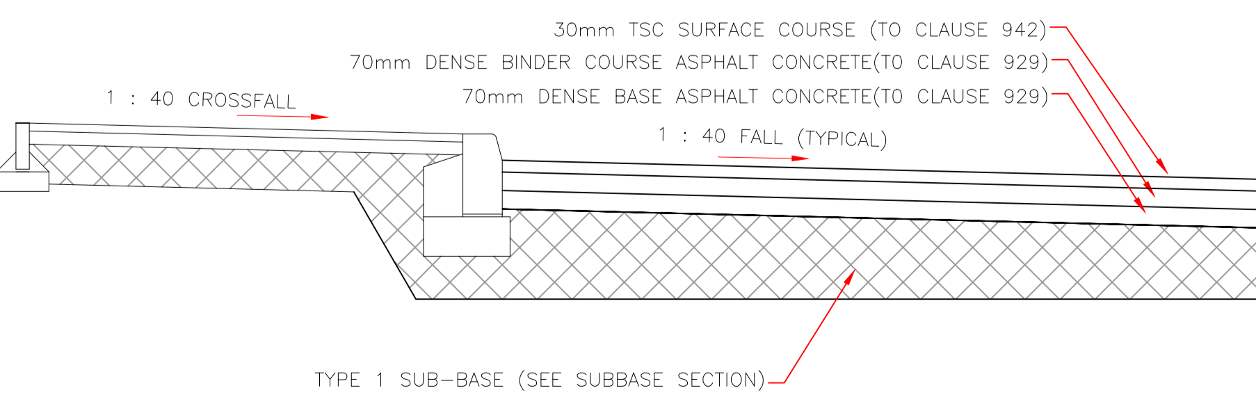
SECTION THROUGH EX. ROAD AT NEW JUNCTION
