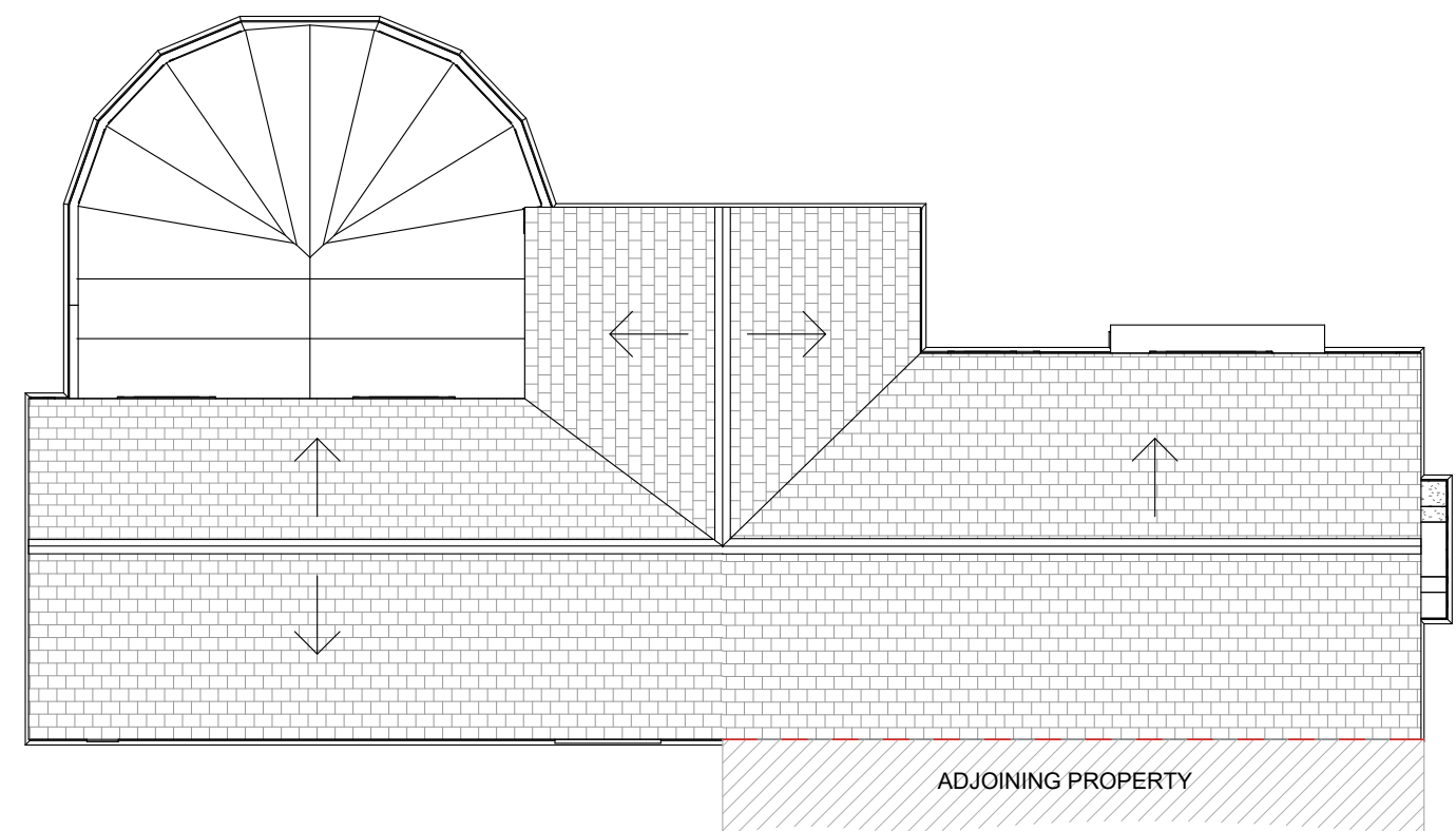
3 Existing Roof Level 1 : 100
