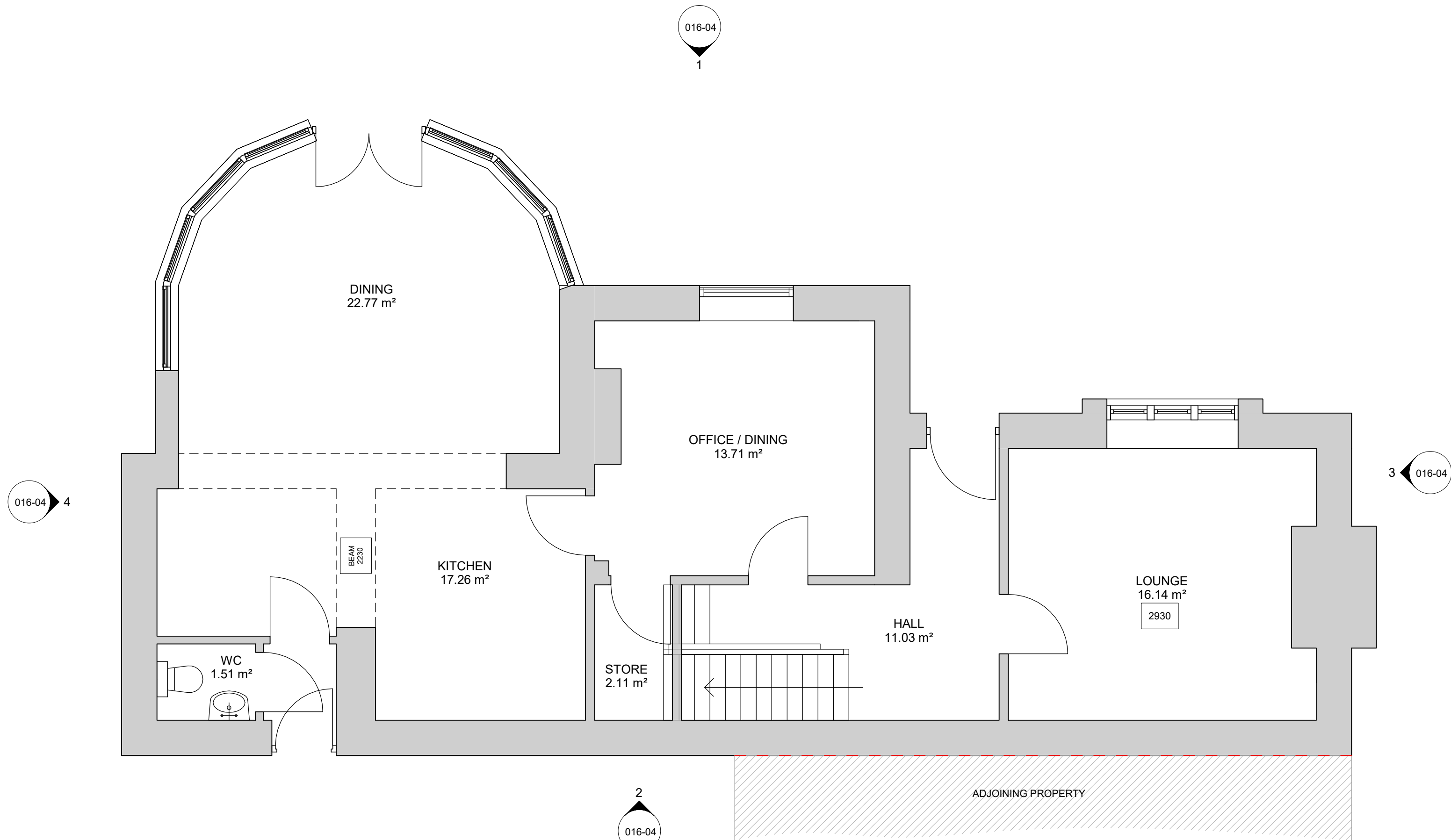
1 Existing Ground Floor Level 1 : 50
