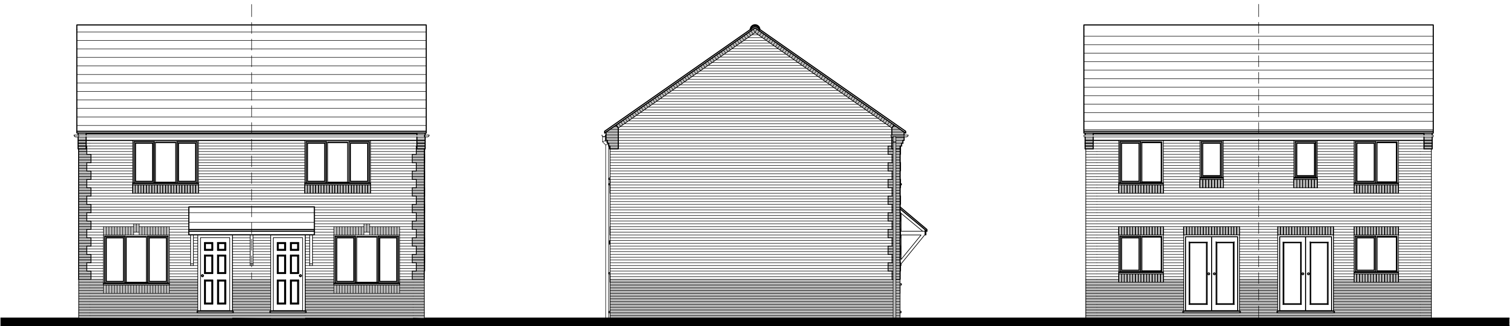
FRONT ELEVATION
