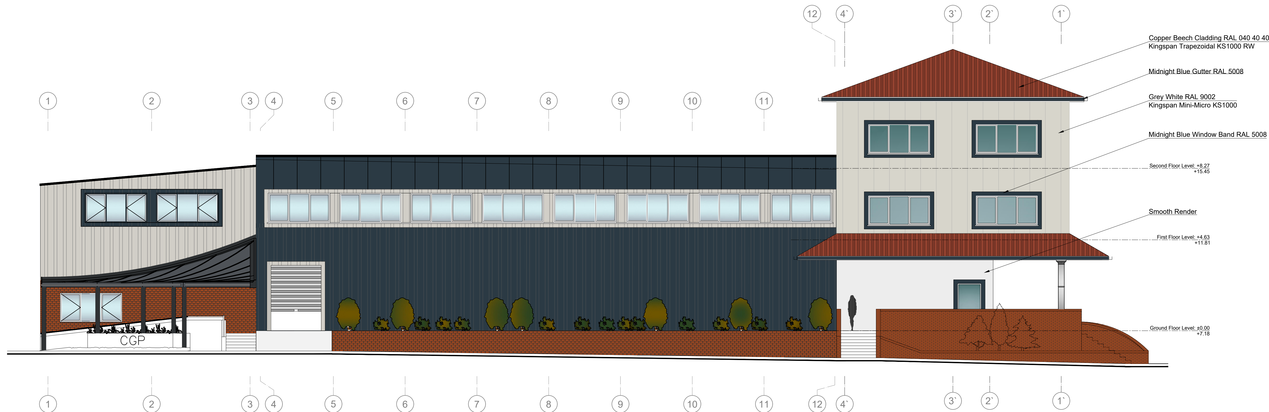
2 PROPOSED WESTERN ELEVATION Scale 1:100
