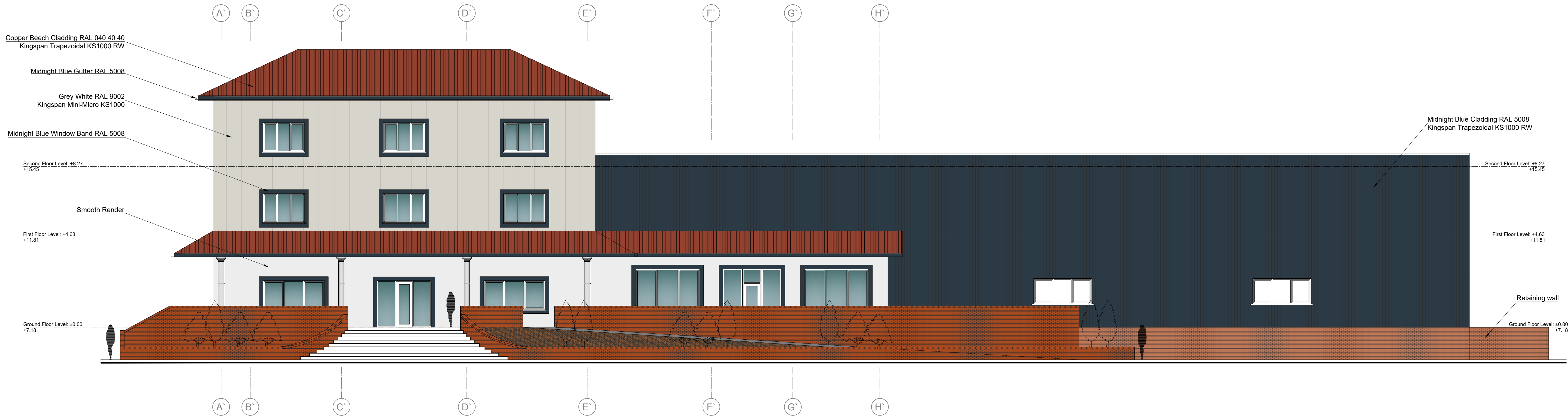
1 PROPOSED SOUTHERN ELEVATION Scale 1:100
