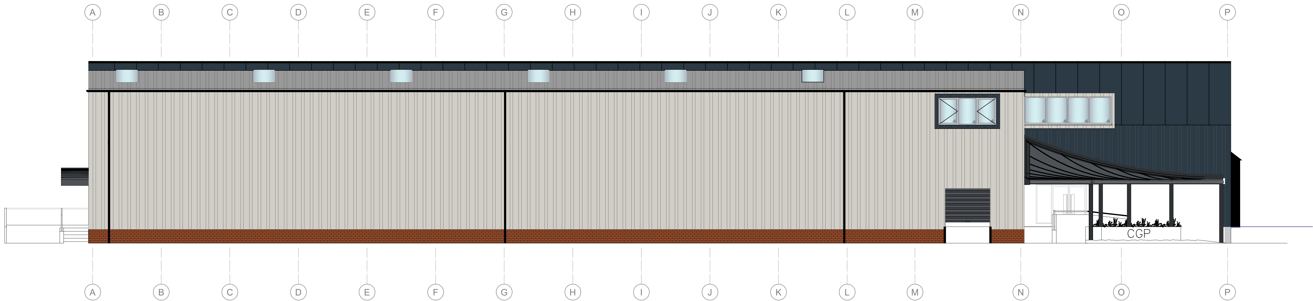
1 EXISTING NORTHERN ELEVATION Scale 1:100
