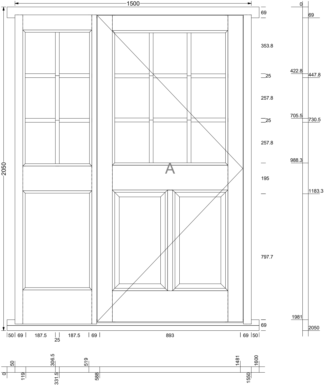
1 X Screen - S2 (Door)
