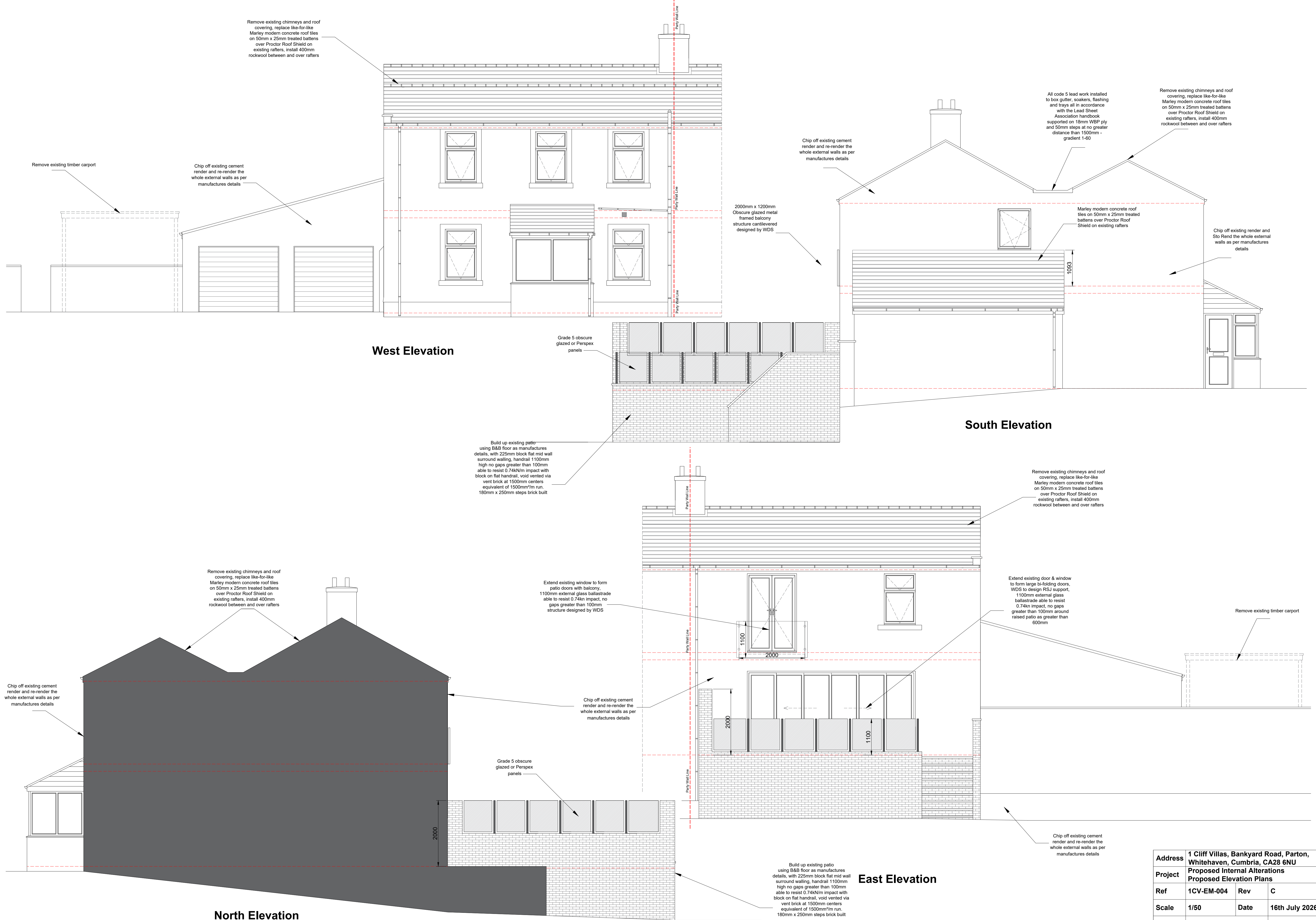
North Elevation
