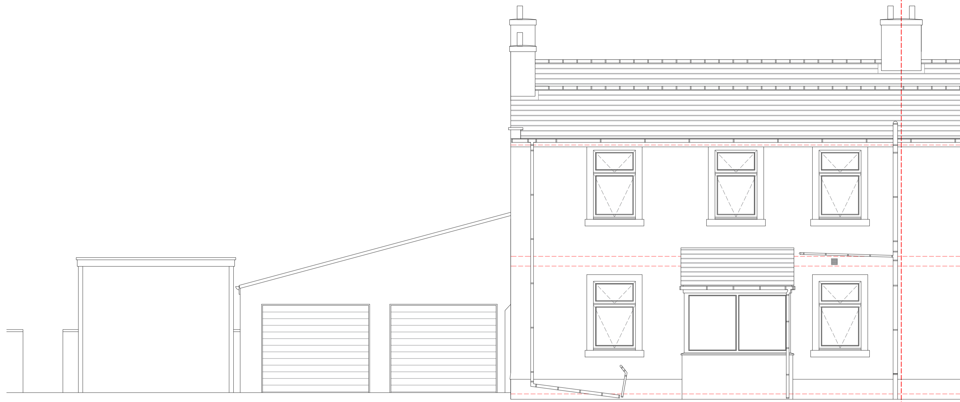
West Elevation
