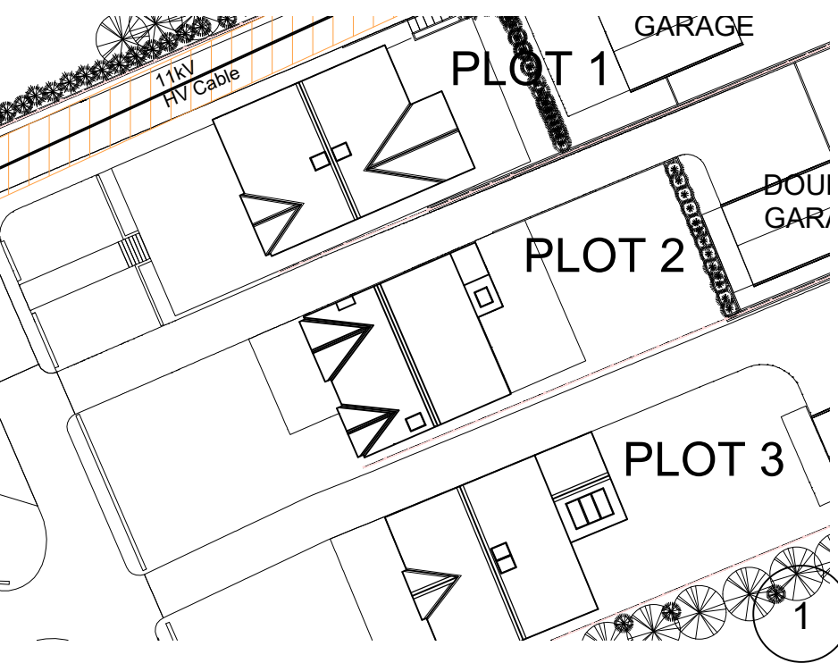
Annotation Site Plan 1:500
