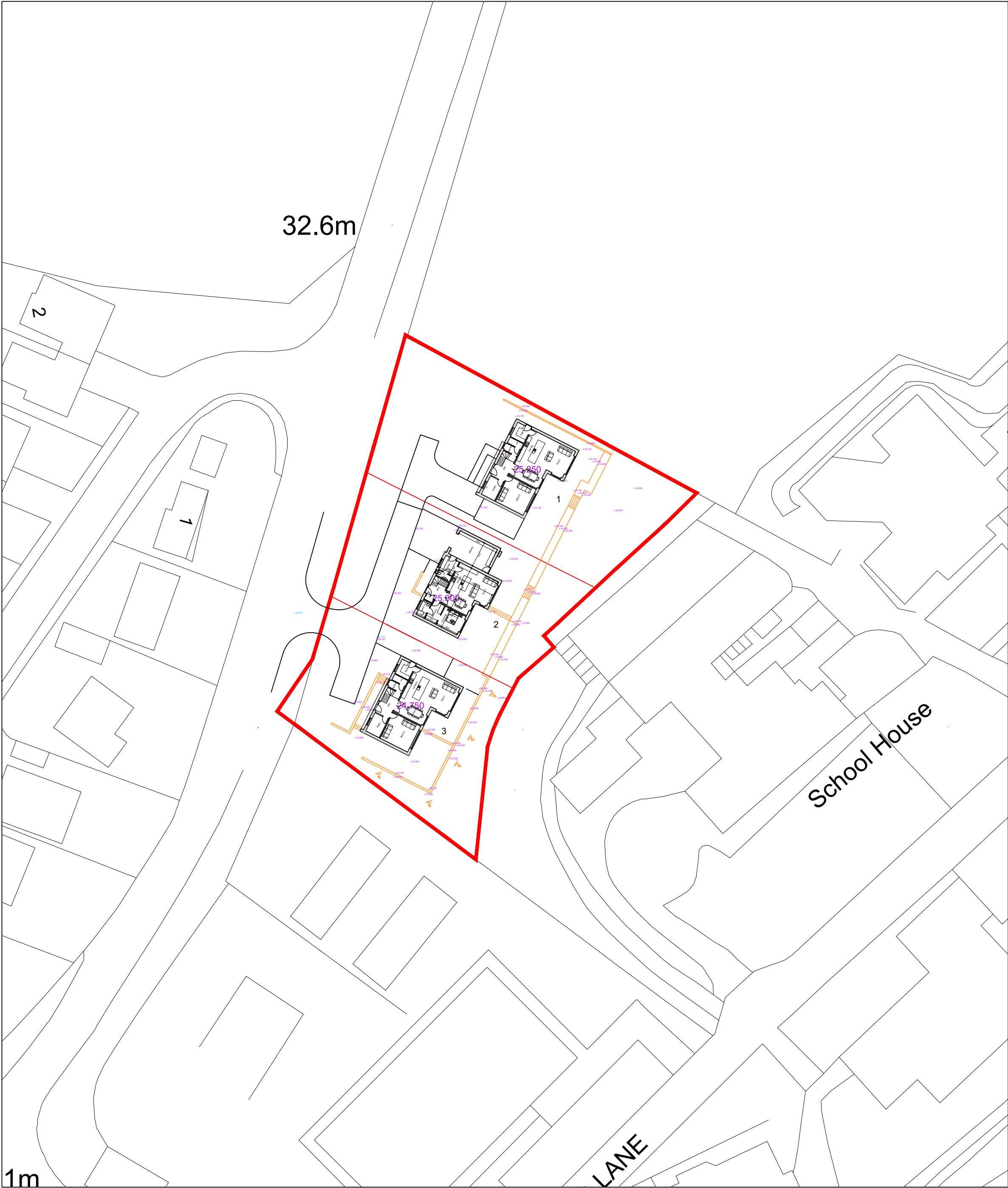
Block Plan
