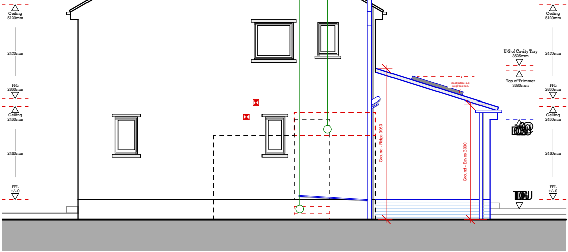
ELEVATION - PROPOSED SIDE SETTING OUT
