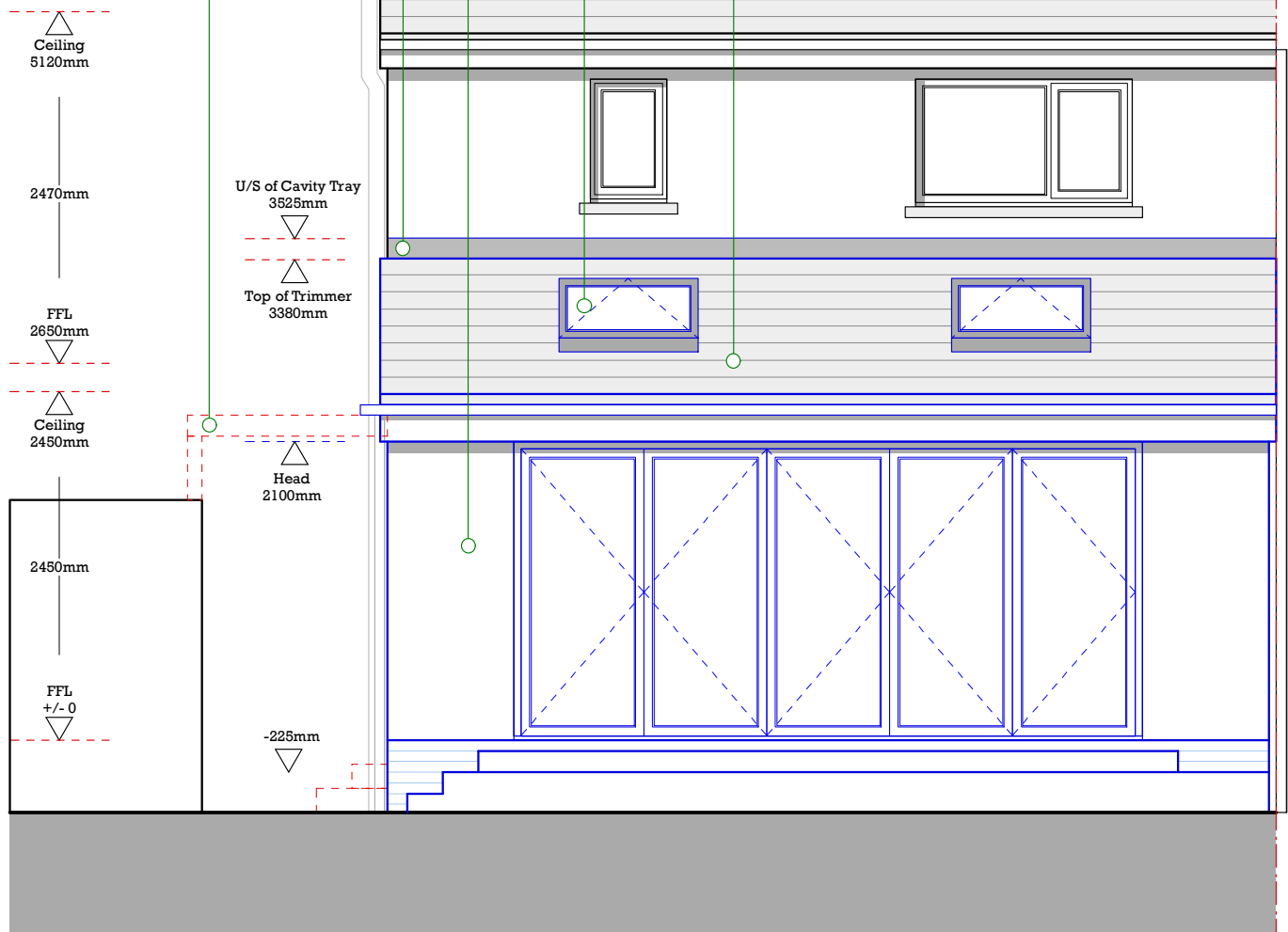
1 ELEVATION - PROPOSED REAR SETTING OUT
