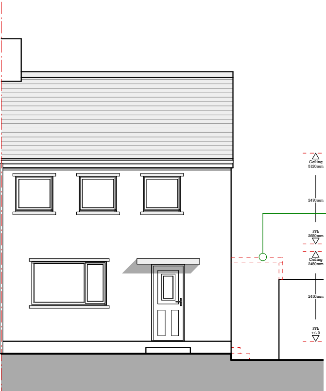
ELEVATION - PROPOSED FRONT SETTING OUT
