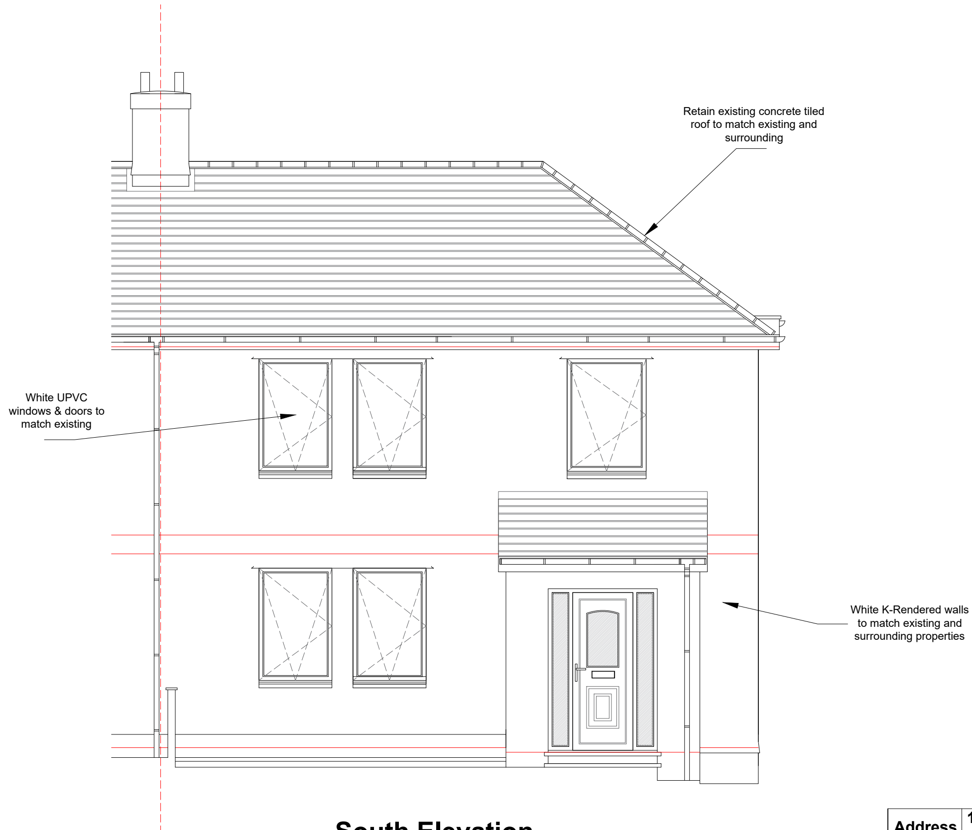
South Elevation
