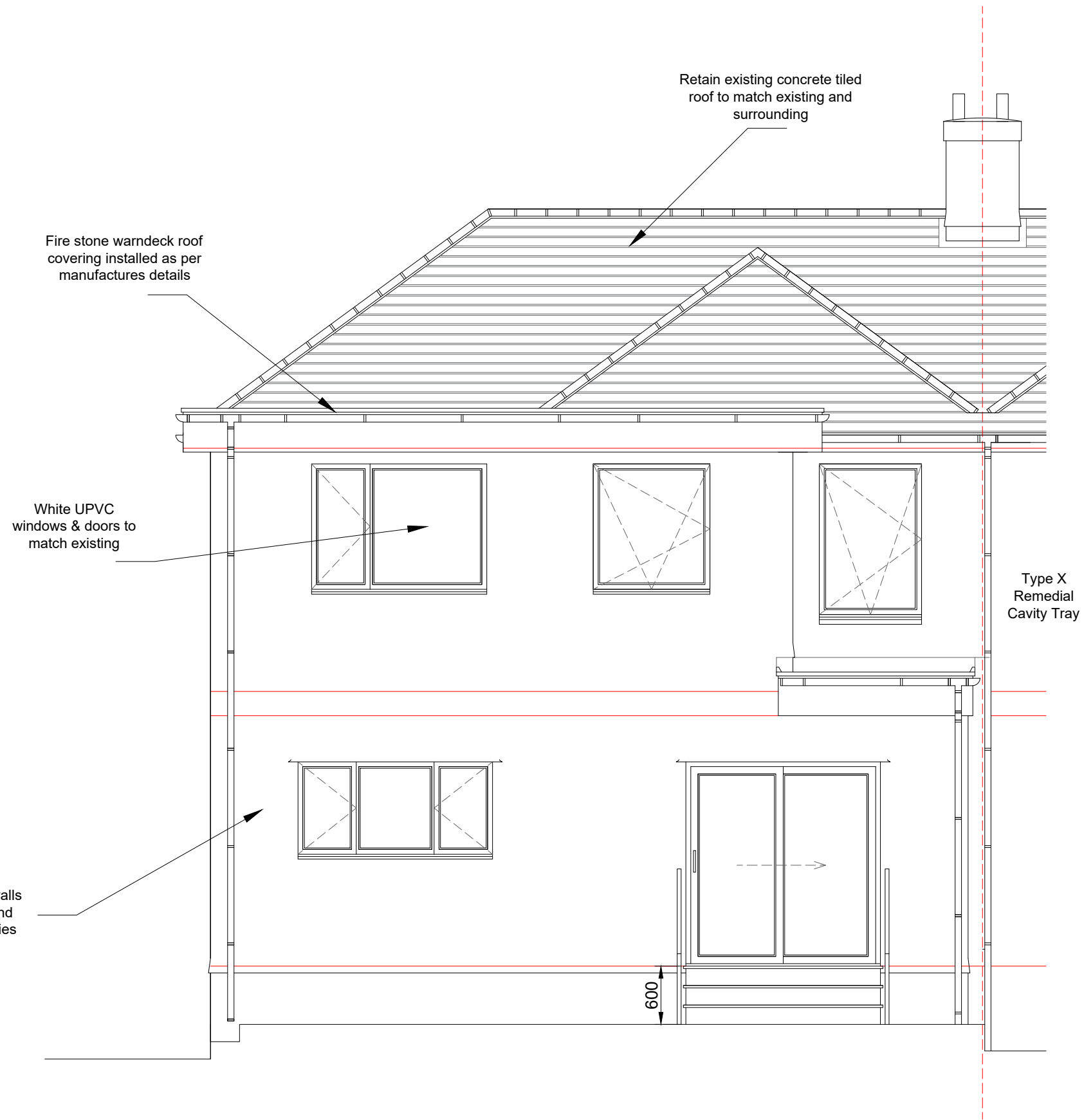
North Elevation
