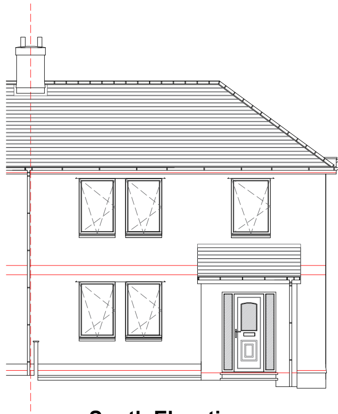
South Elevations
