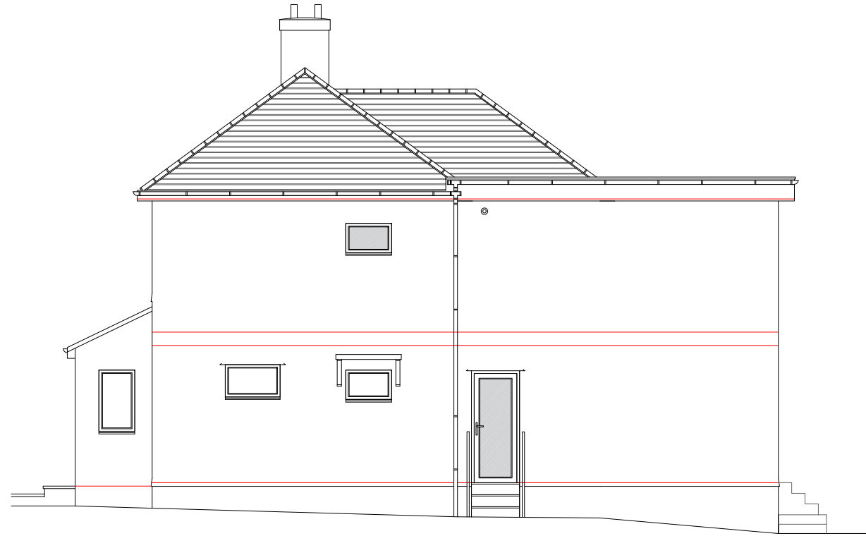
East Elevations
