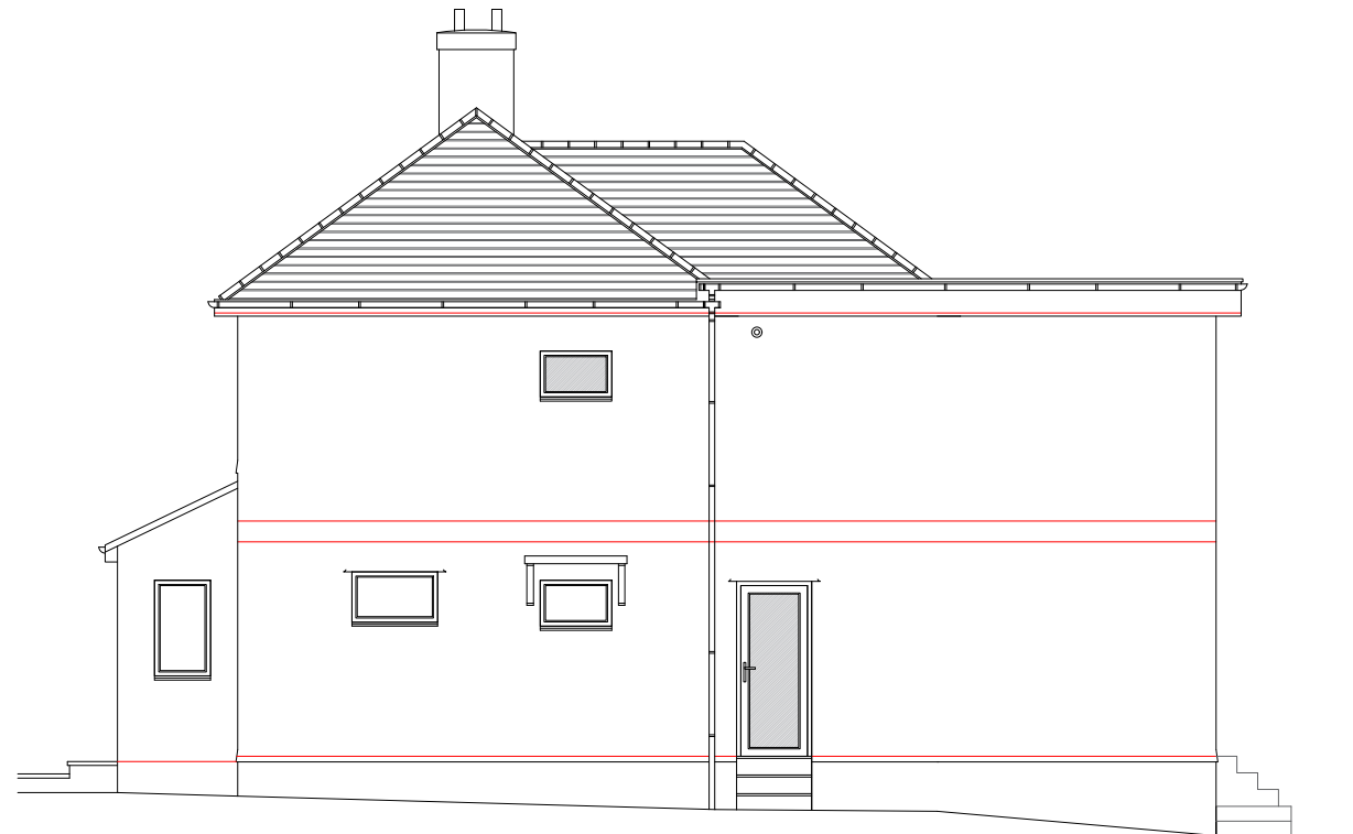
East Elevations
