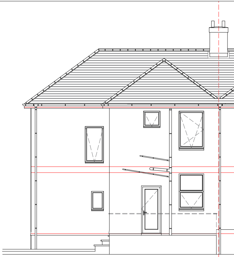
North Elevations
