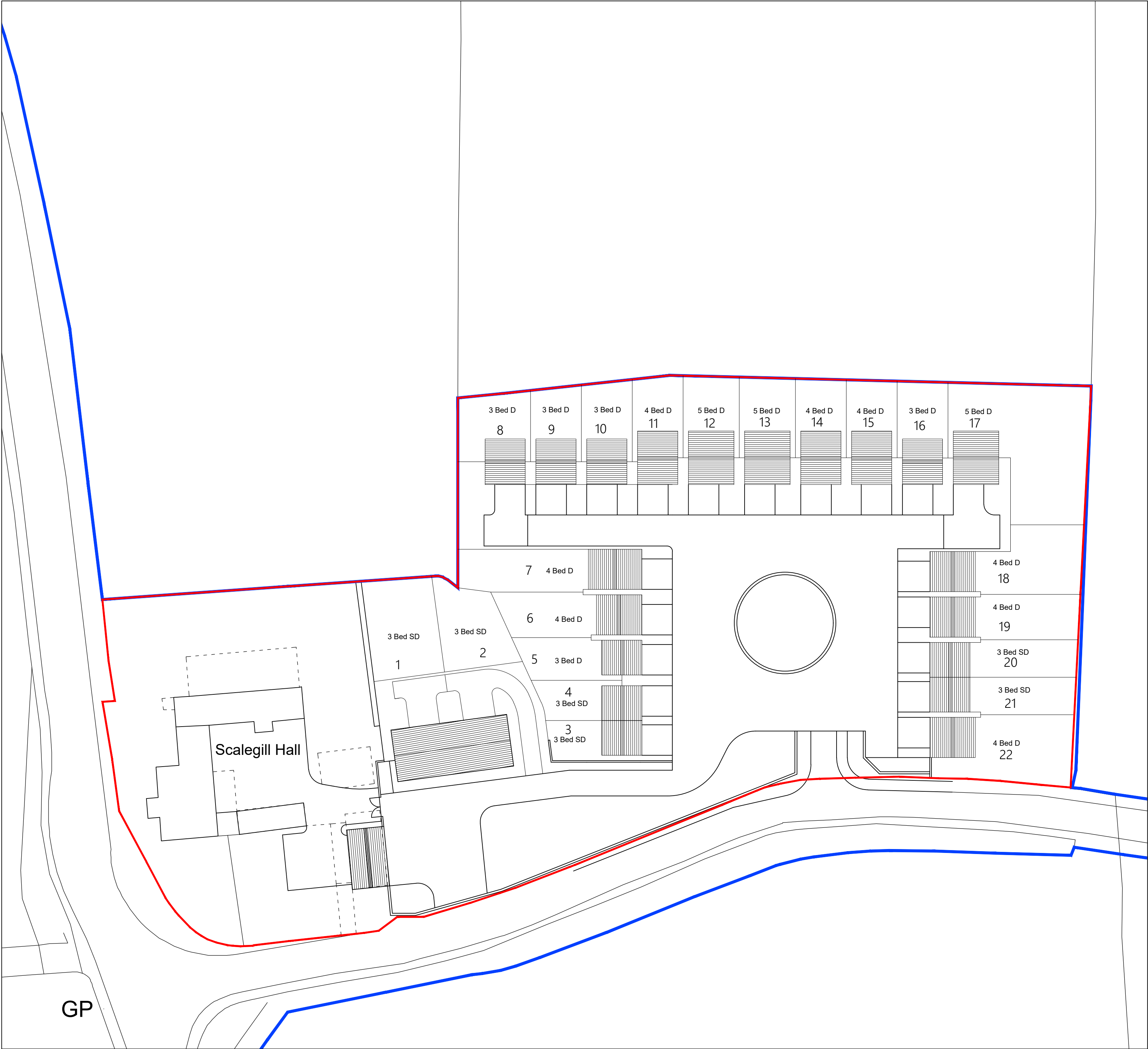
SITE LAYOUT
