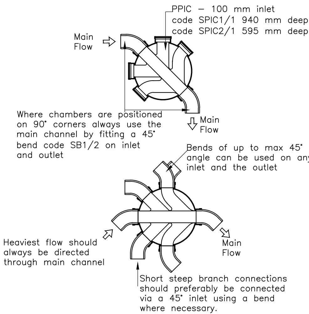
General Plastic Inspection Chamber Plan
