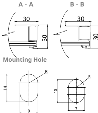
Frame Cross Section
