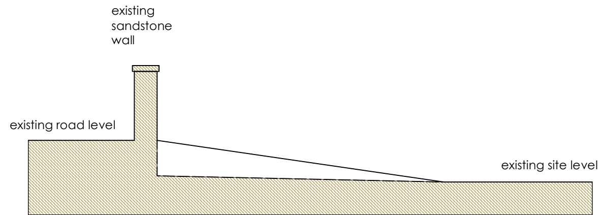
SECTION THROUGH NEW SITE ENTRANCE 1 : 100
