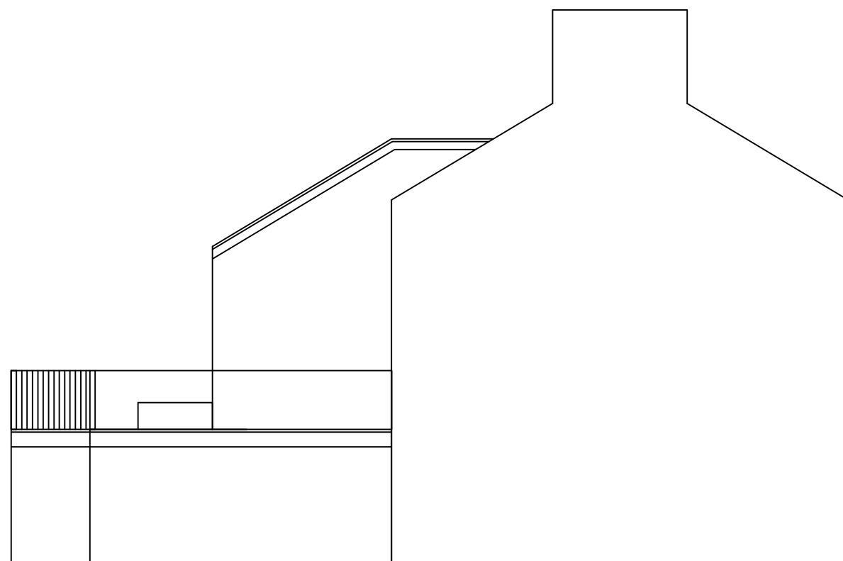
Proposed Gable Elevation 2
