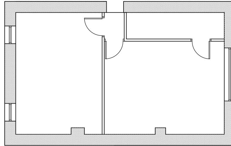
EXISTING FIRST FLOOR LAYOUT 1.100
