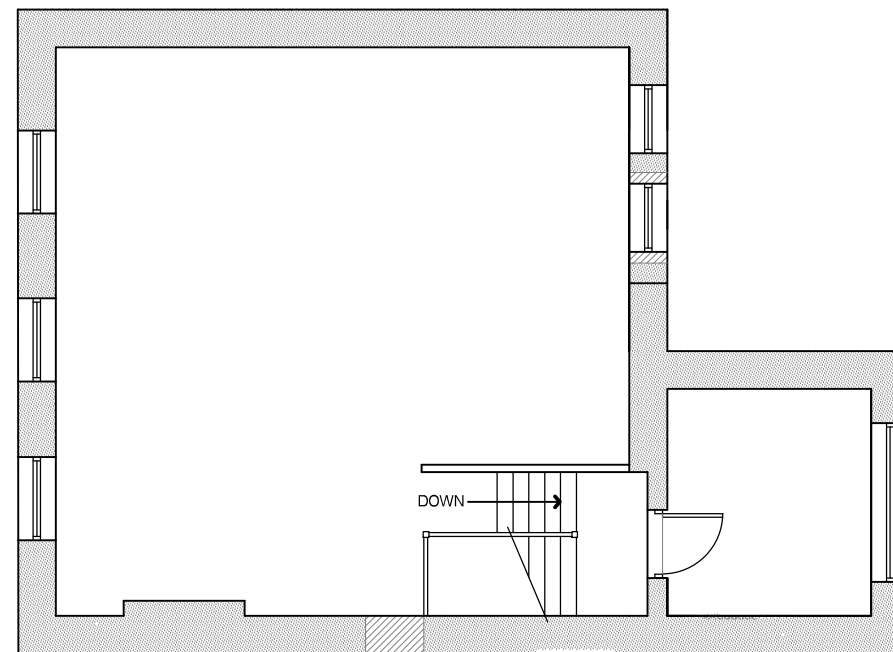
PROPOSED FIRST FLOOR LAYOUT 1.100
