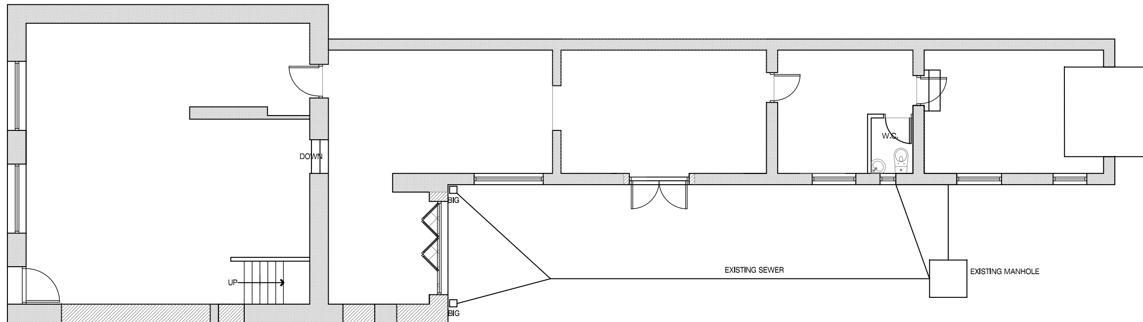
PROPOSED GROUND FLOOR LAYOUT 1.100
