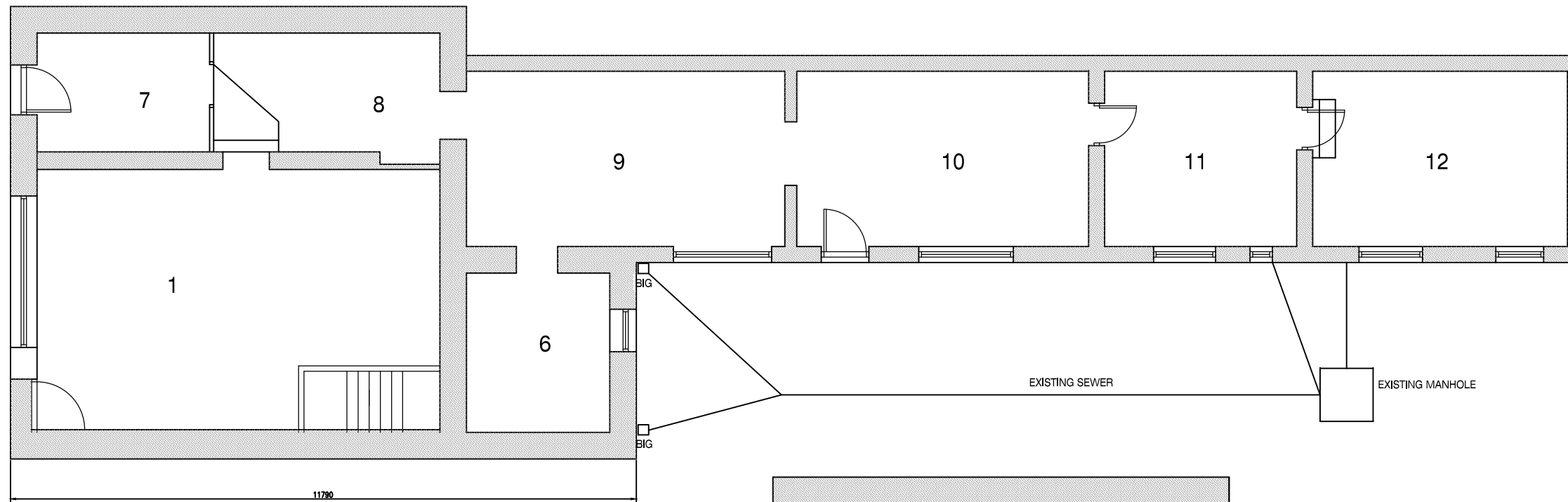
EXISTING GROUND FLOOR LAYOUT 1.100
