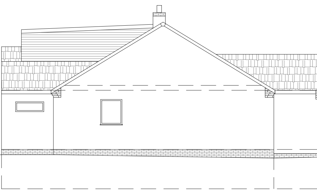
Proposed Side (North West) Elevation
