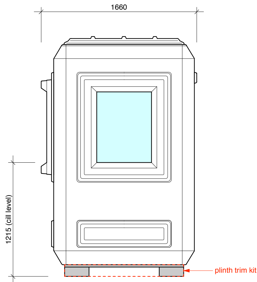
ELEVATION 'A'
