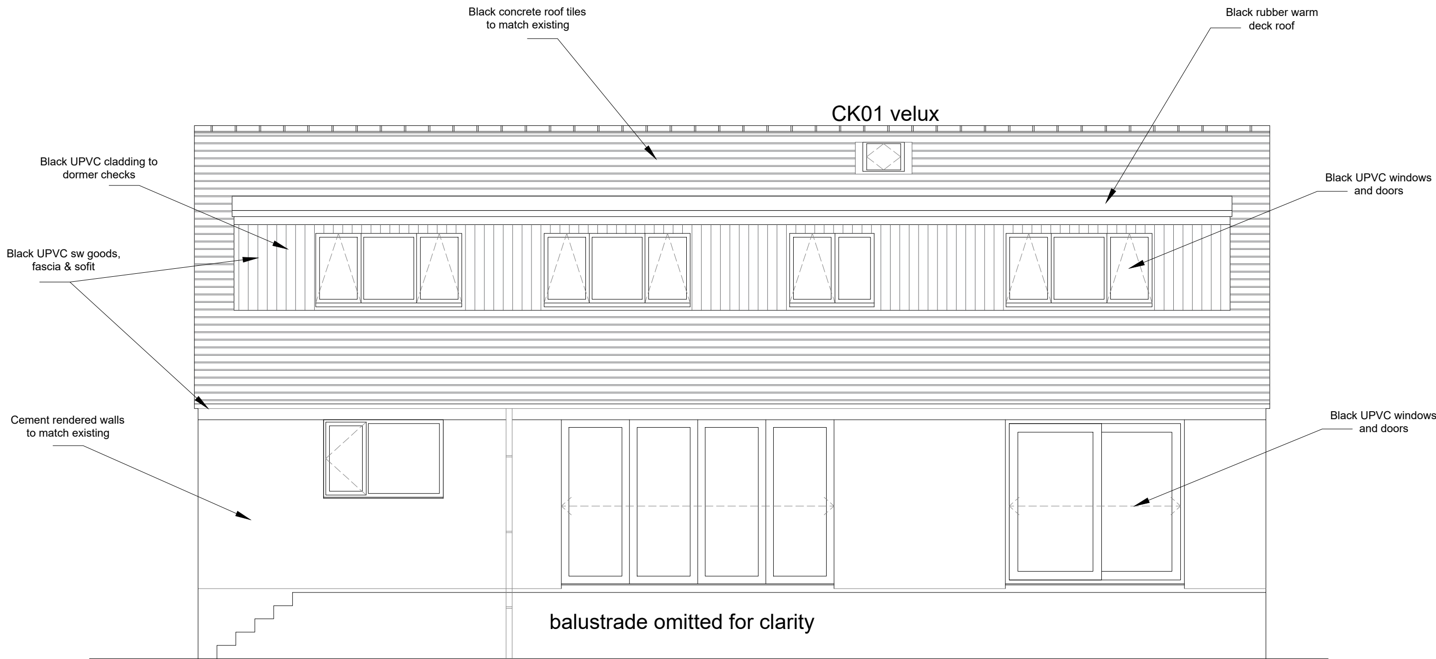
East Elevation
