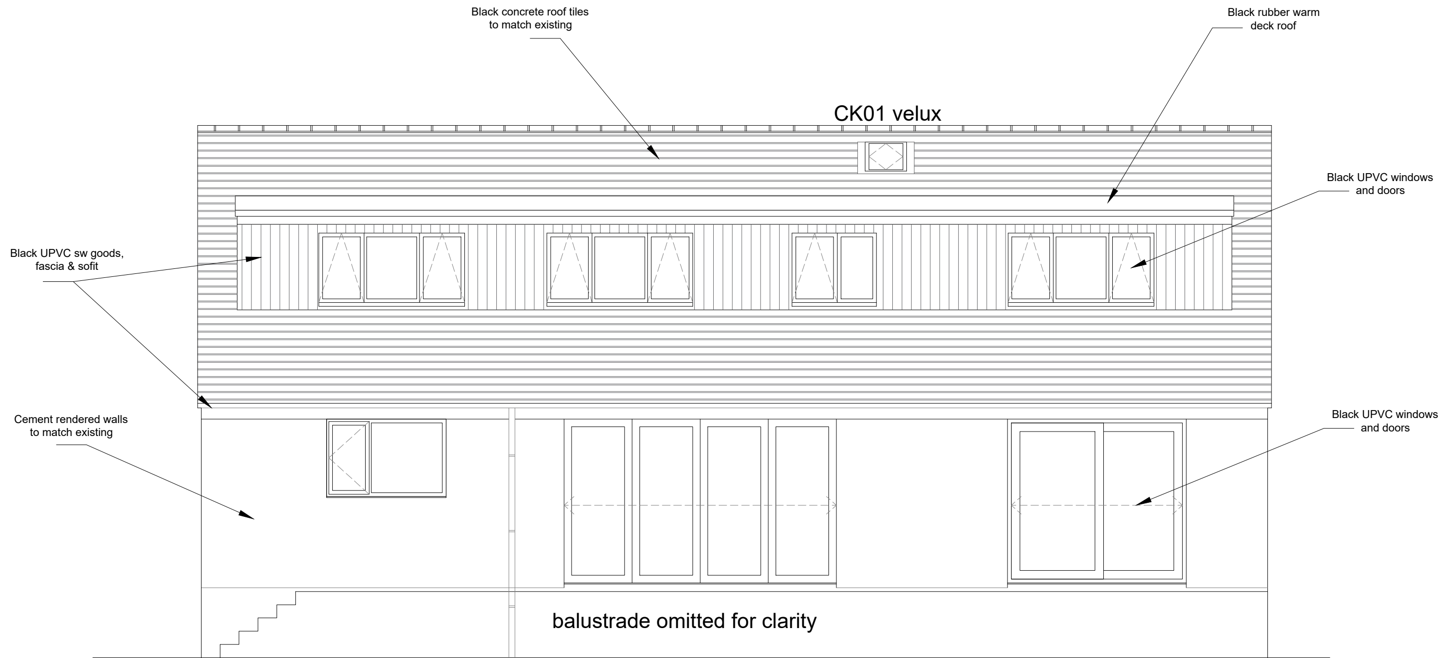
East Elevation
