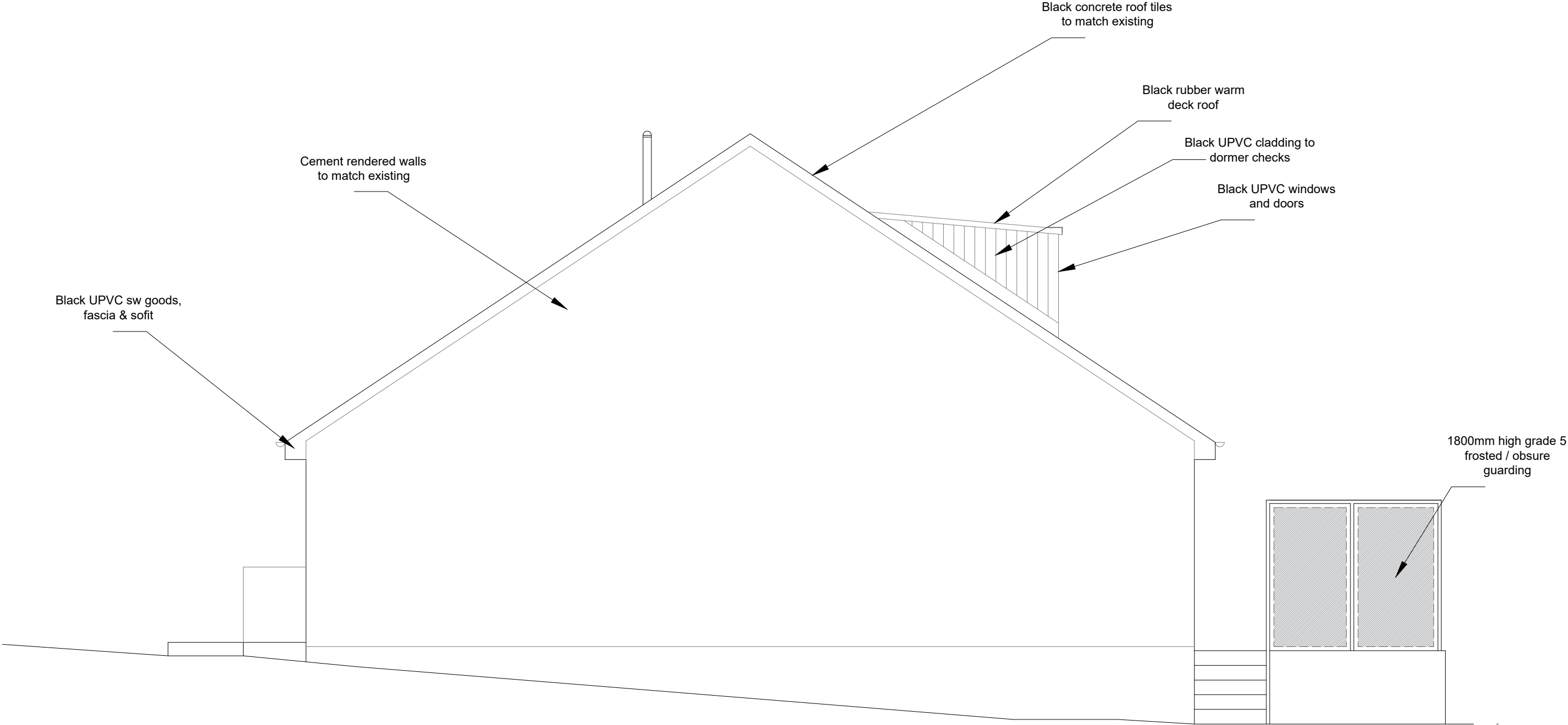
South Elevation
