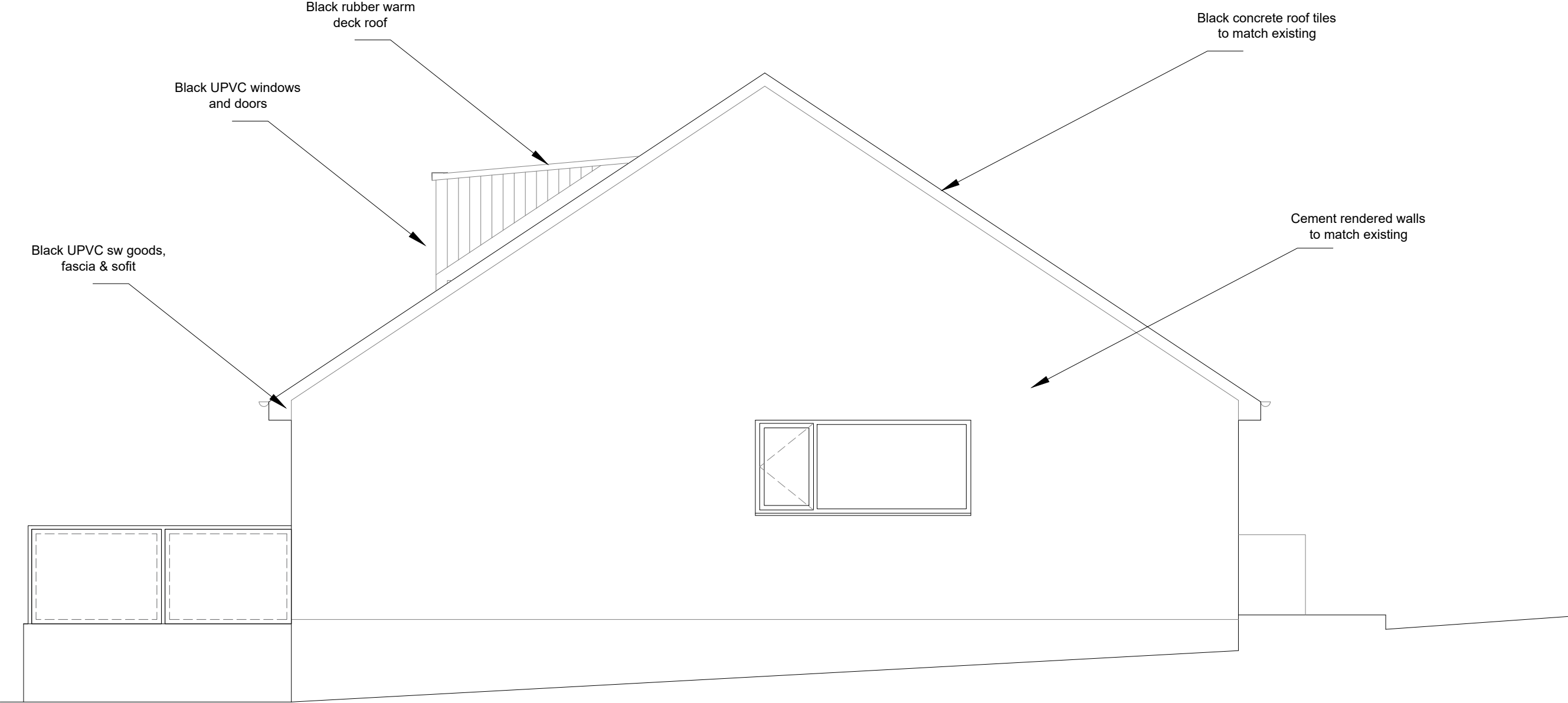
North Elevation
