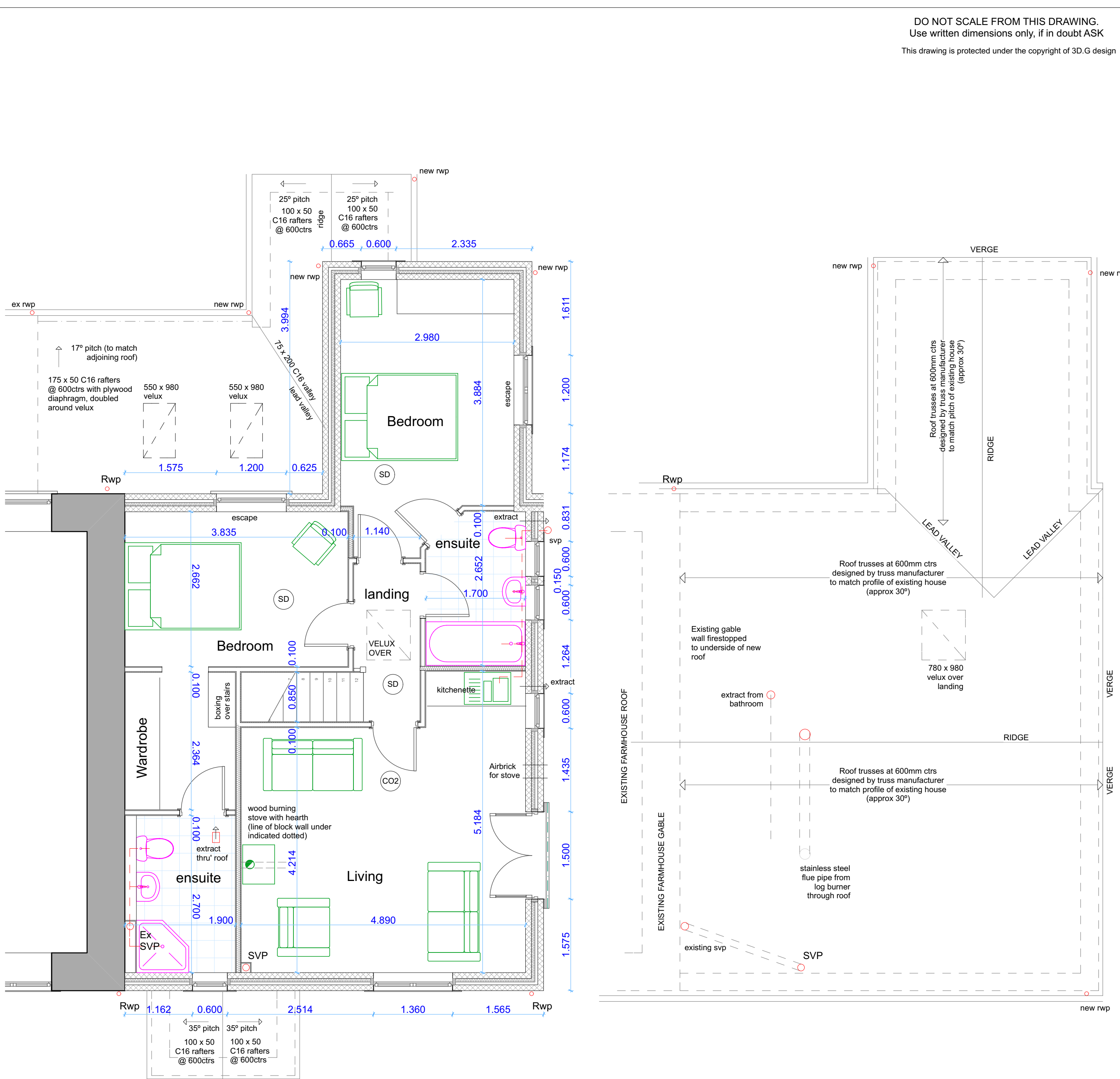
Roof Plan
