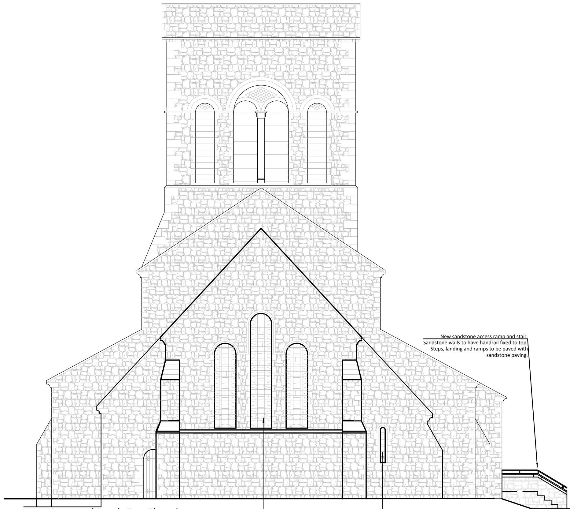
Proposed North East Elevation (no proposed changes) Scale 1:100
