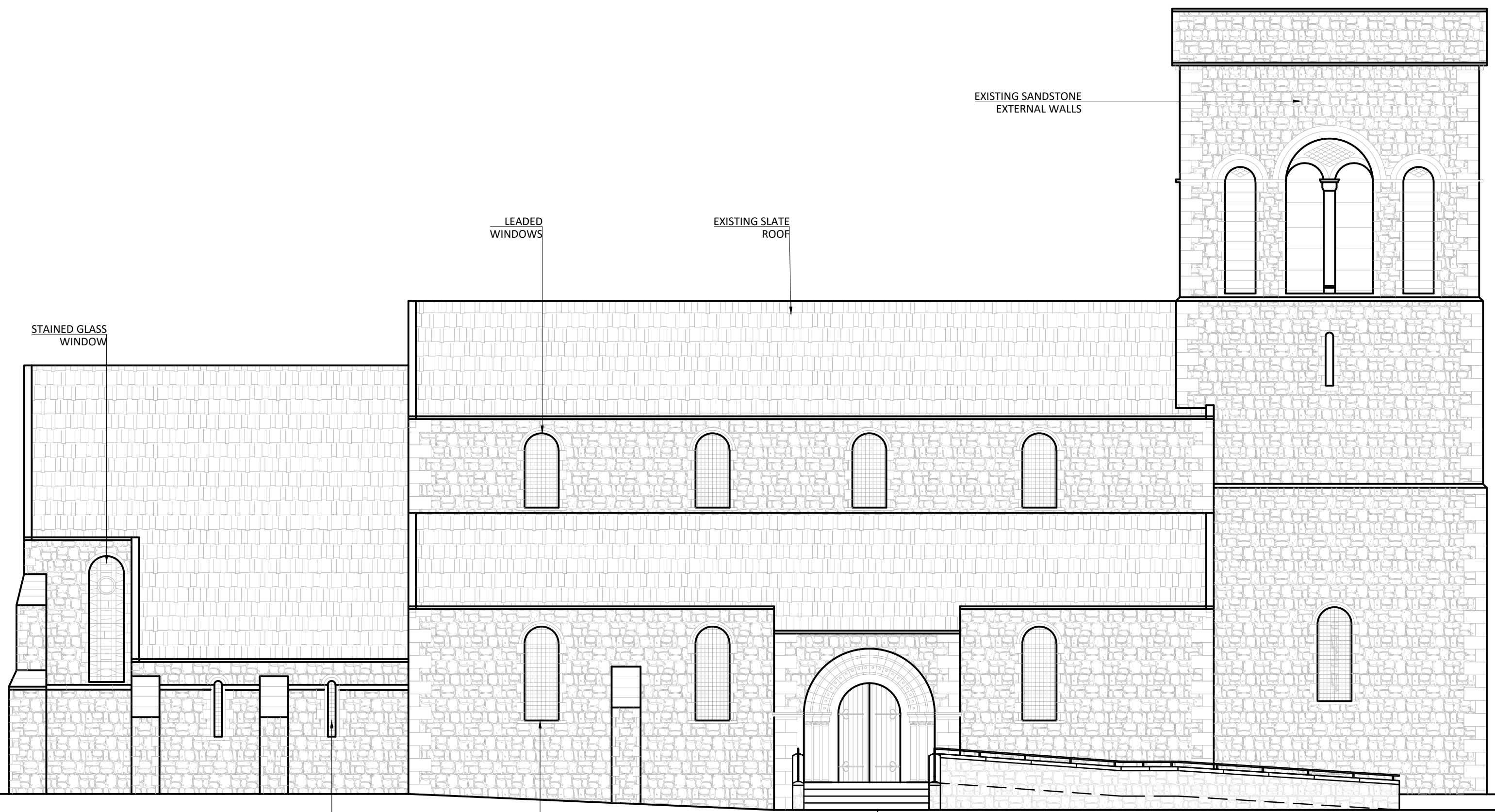
Proposed North West Elevation Scale 1:100
