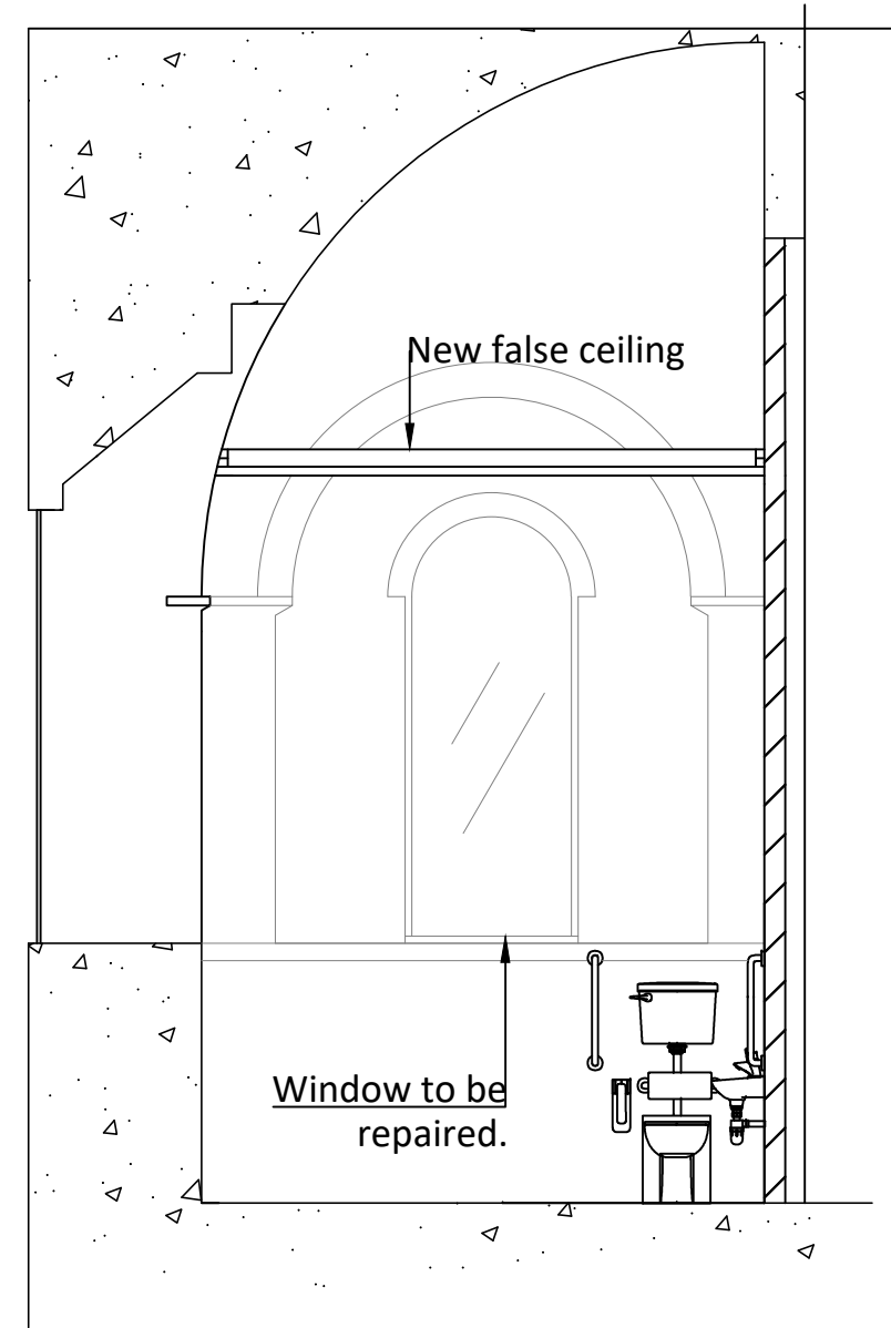
Internal Elevation E (Proposed)
