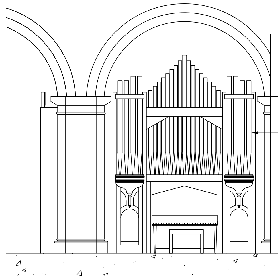
Internal Elevation B (Existing)
