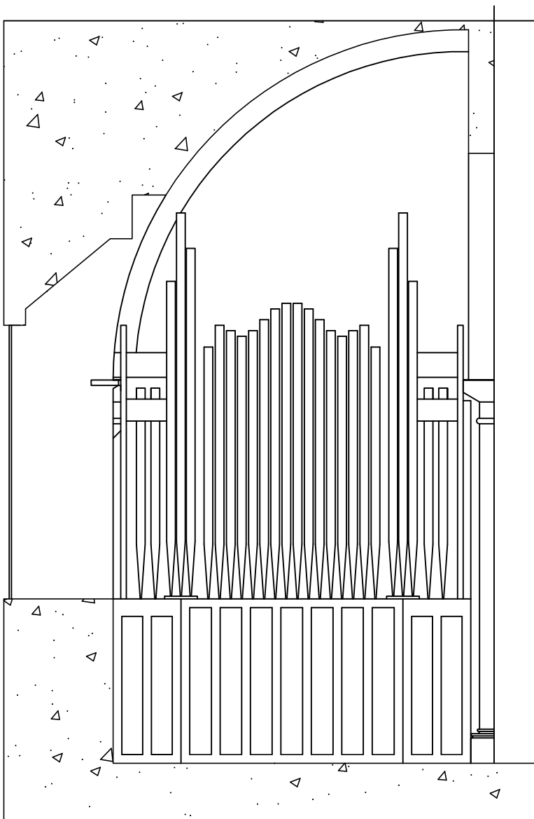
Internal Elevation A (Existing)
