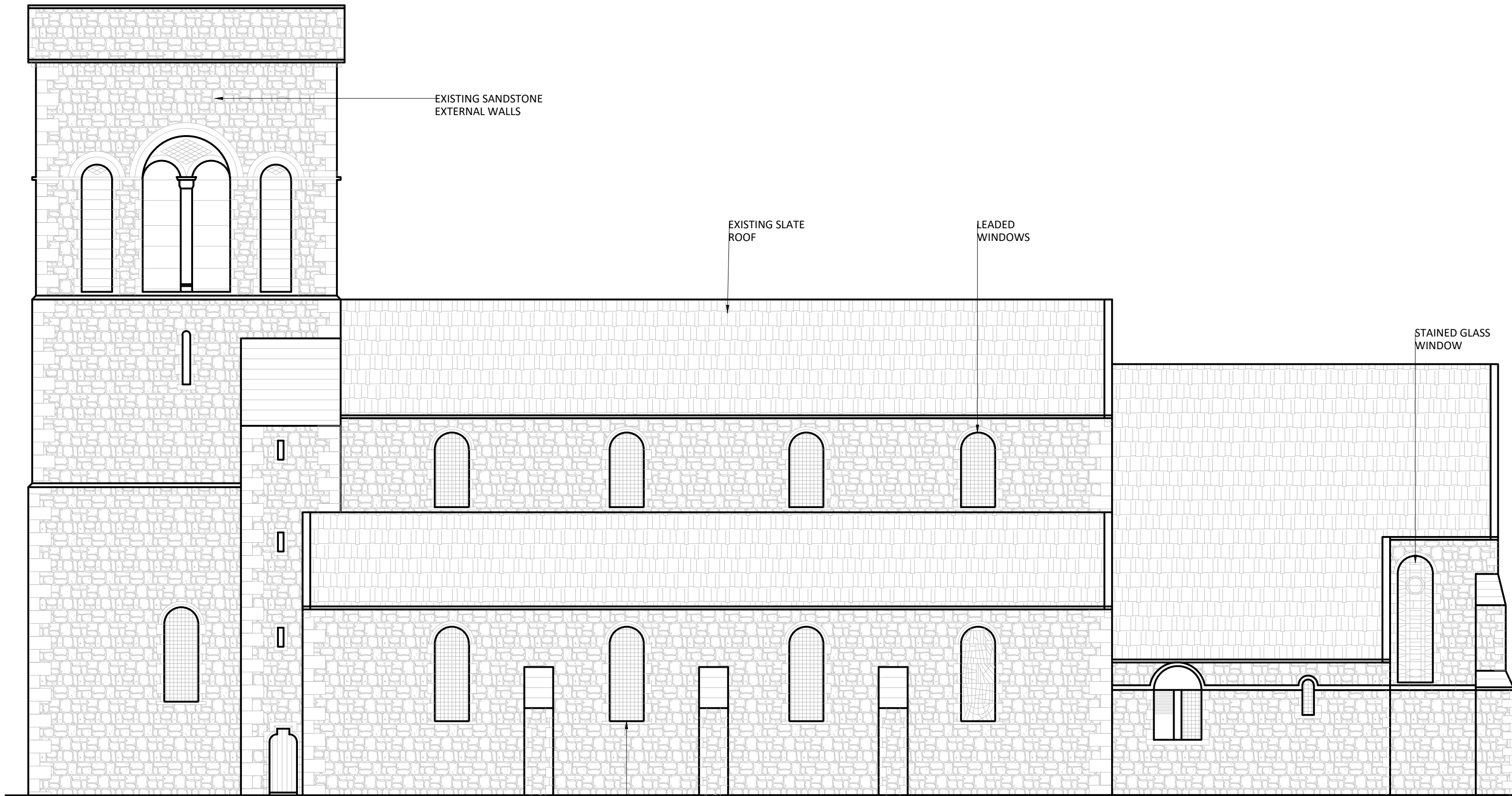
Existing South East Elevation Scale 1:100
