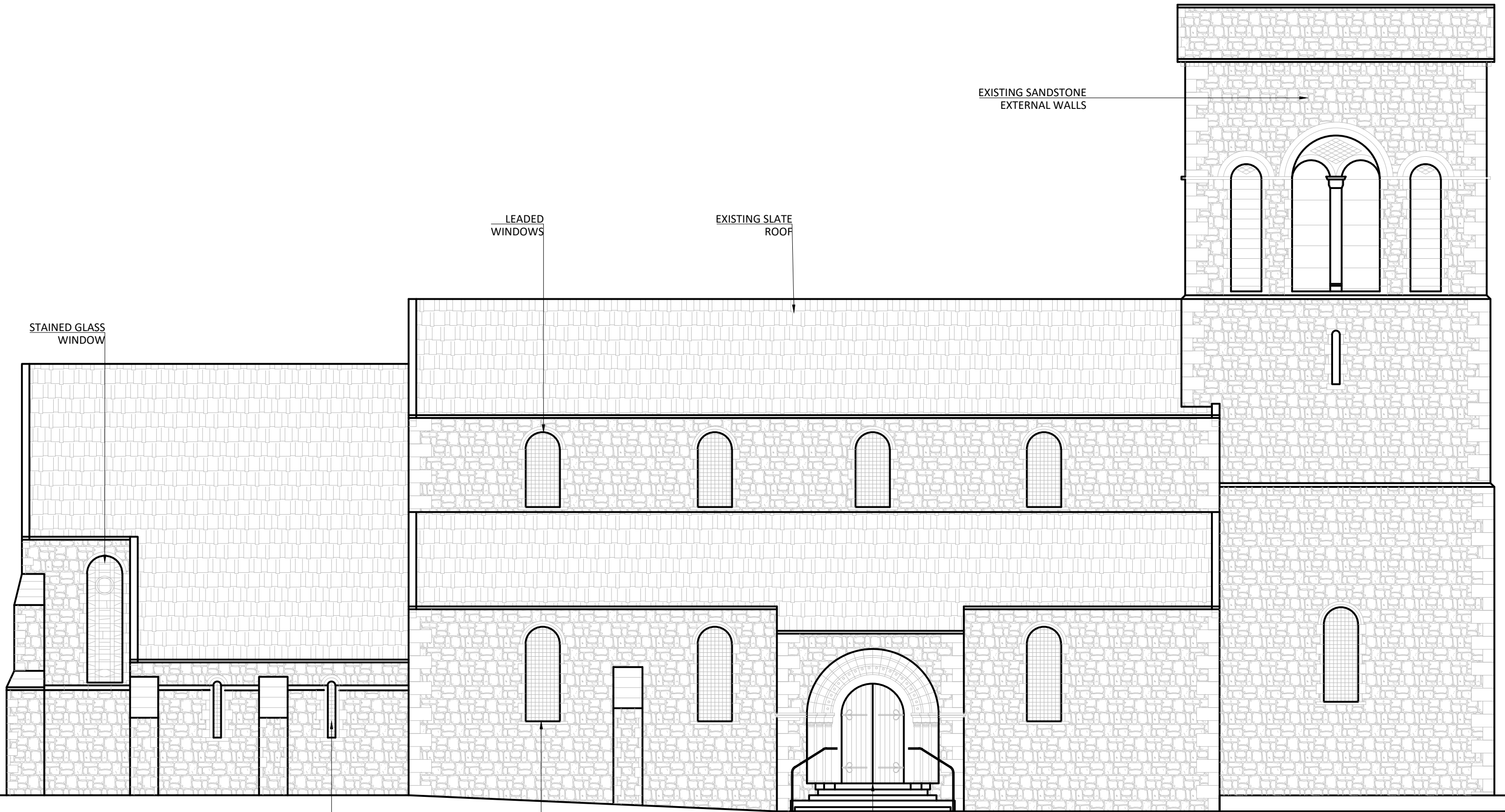
Existing North West Elevation Scale 1:100
