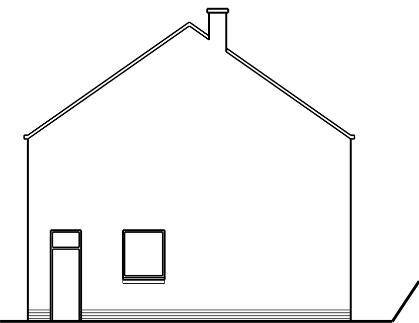
proposed end elevation (north)
