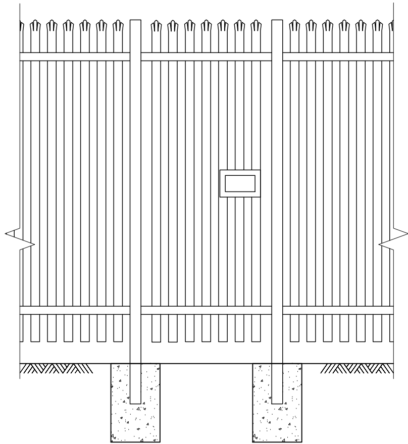
TYPICAL PALISADE FENCE ELEVATION (DOUBLE VEHICLE GATE)
