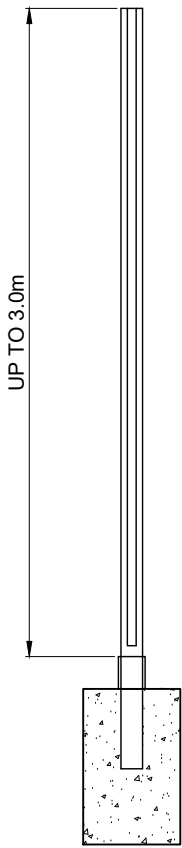
TYPICAL CROSS SECTION
