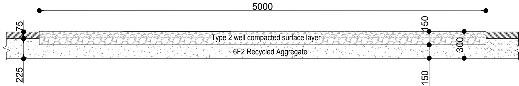
Made Track Type 2 Detail 1 : 25
