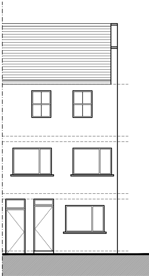
Existing Front Elevation Scale 1:100
