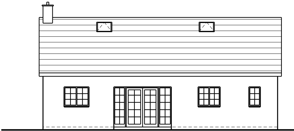
existing rear elevation (SE)
