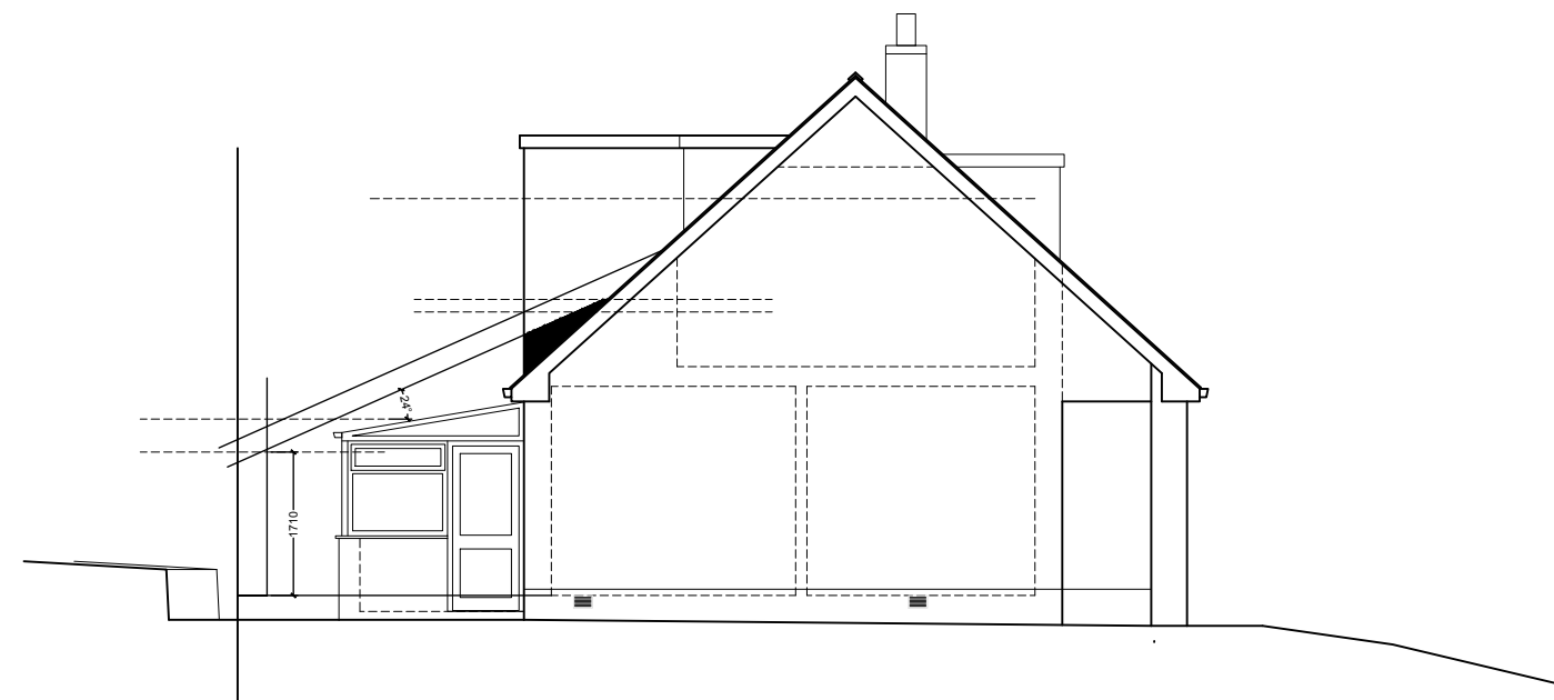
Side (N) Elevation
