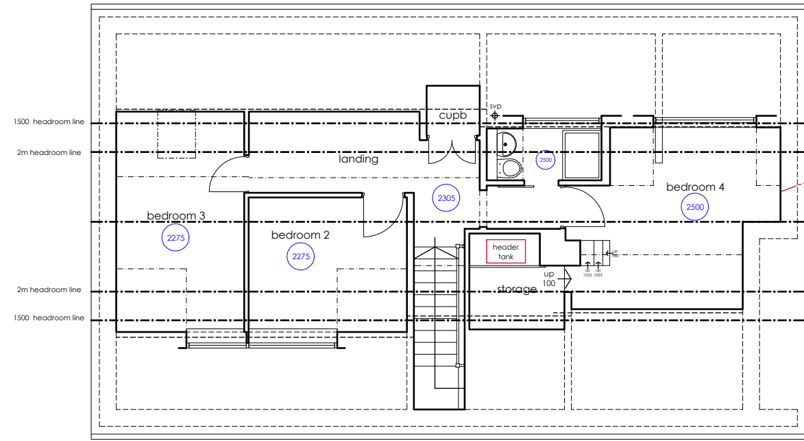
Attic Floor
