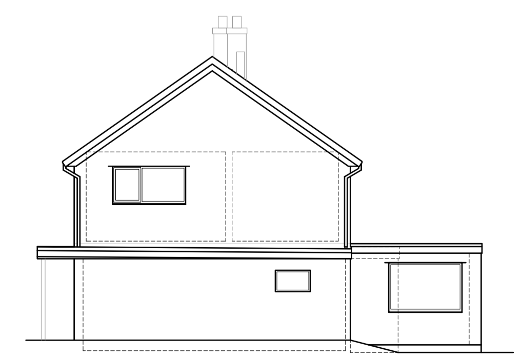
Side (NE) Elevation
