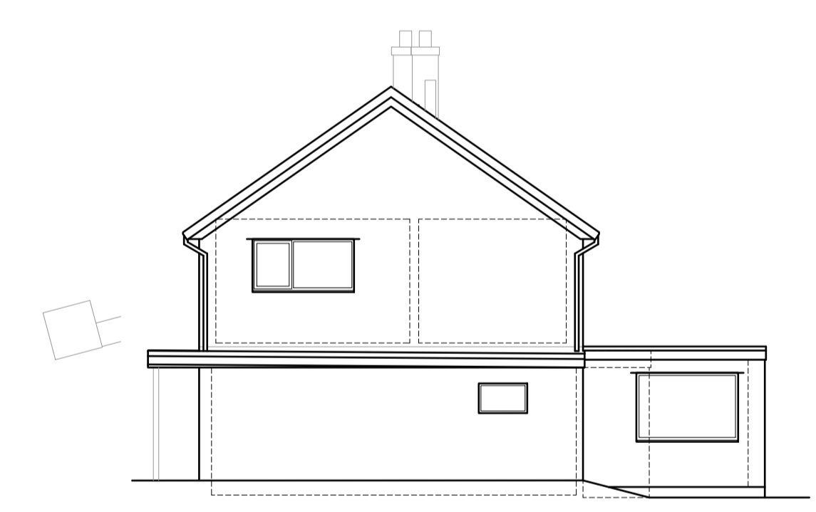
Side (NE) Elevation
