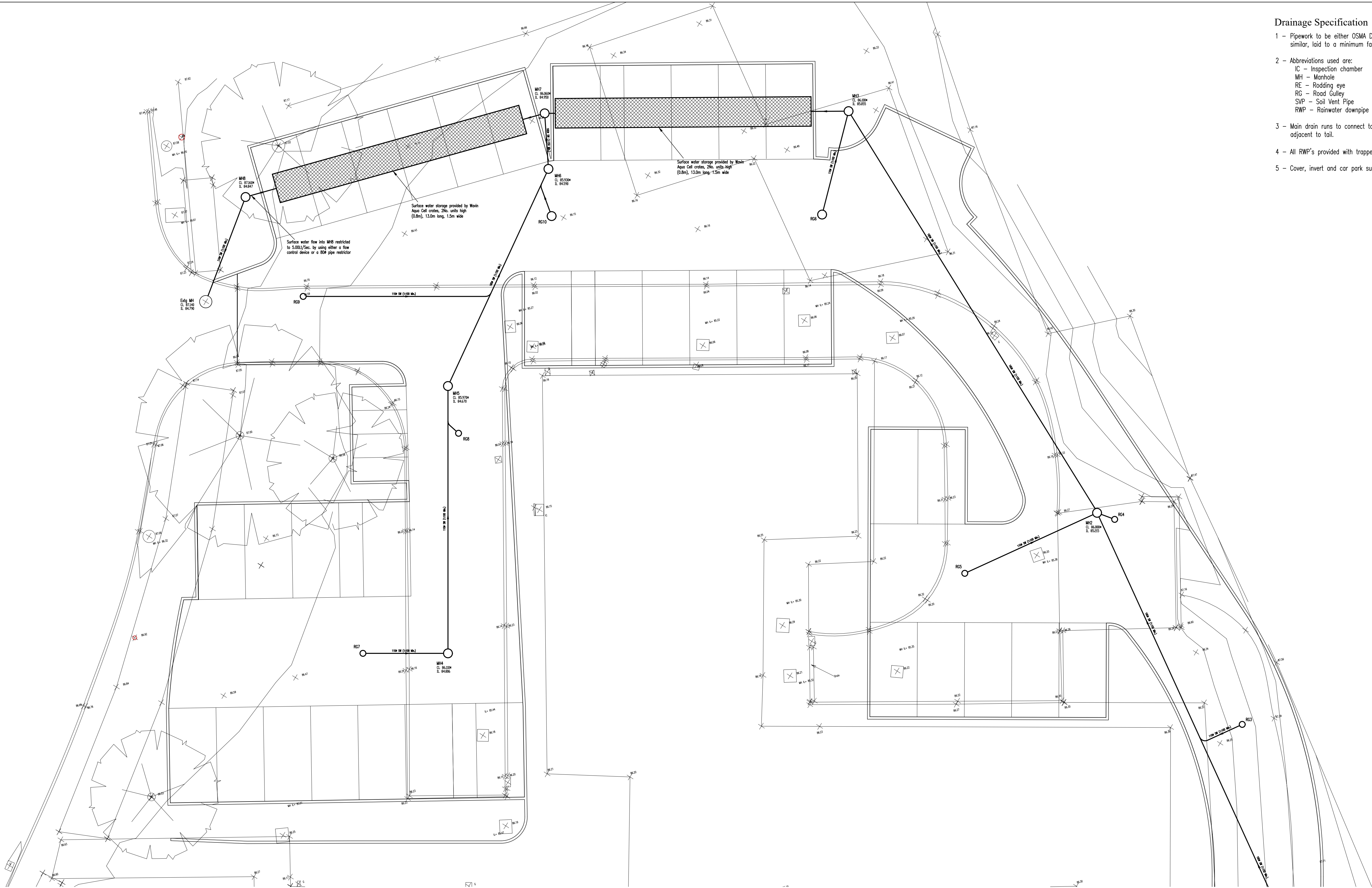
Proposed Drainage Layout - Sheet No. 2 of 2 Scale 1:100
